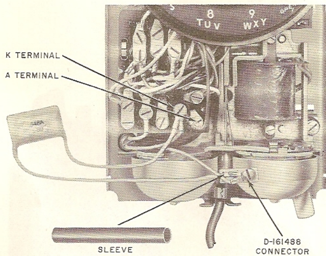
Fig. 22 — Replacing Capacitor
