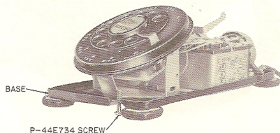
Fig. 8 — 500-Type Telephone Set, Housing Assembly
