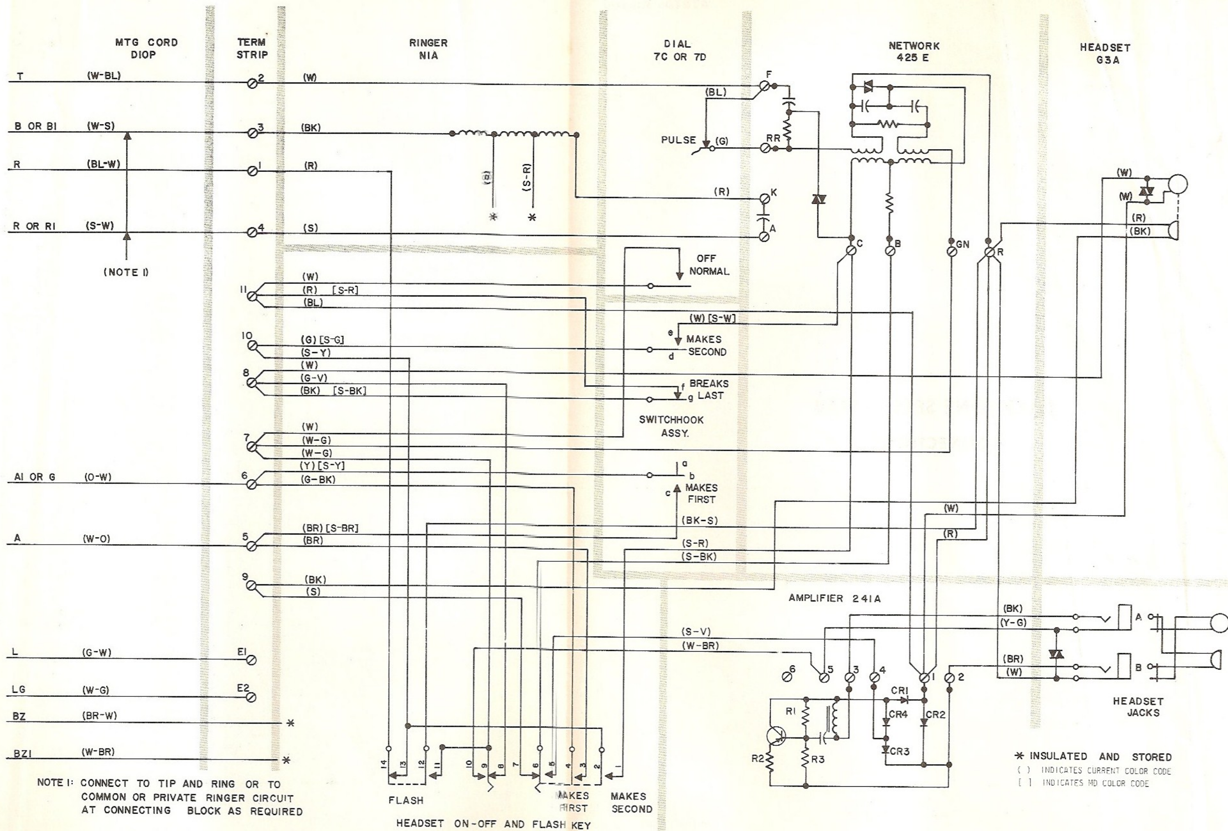
Fig. 1 - 514B Telephone Set, Connections
