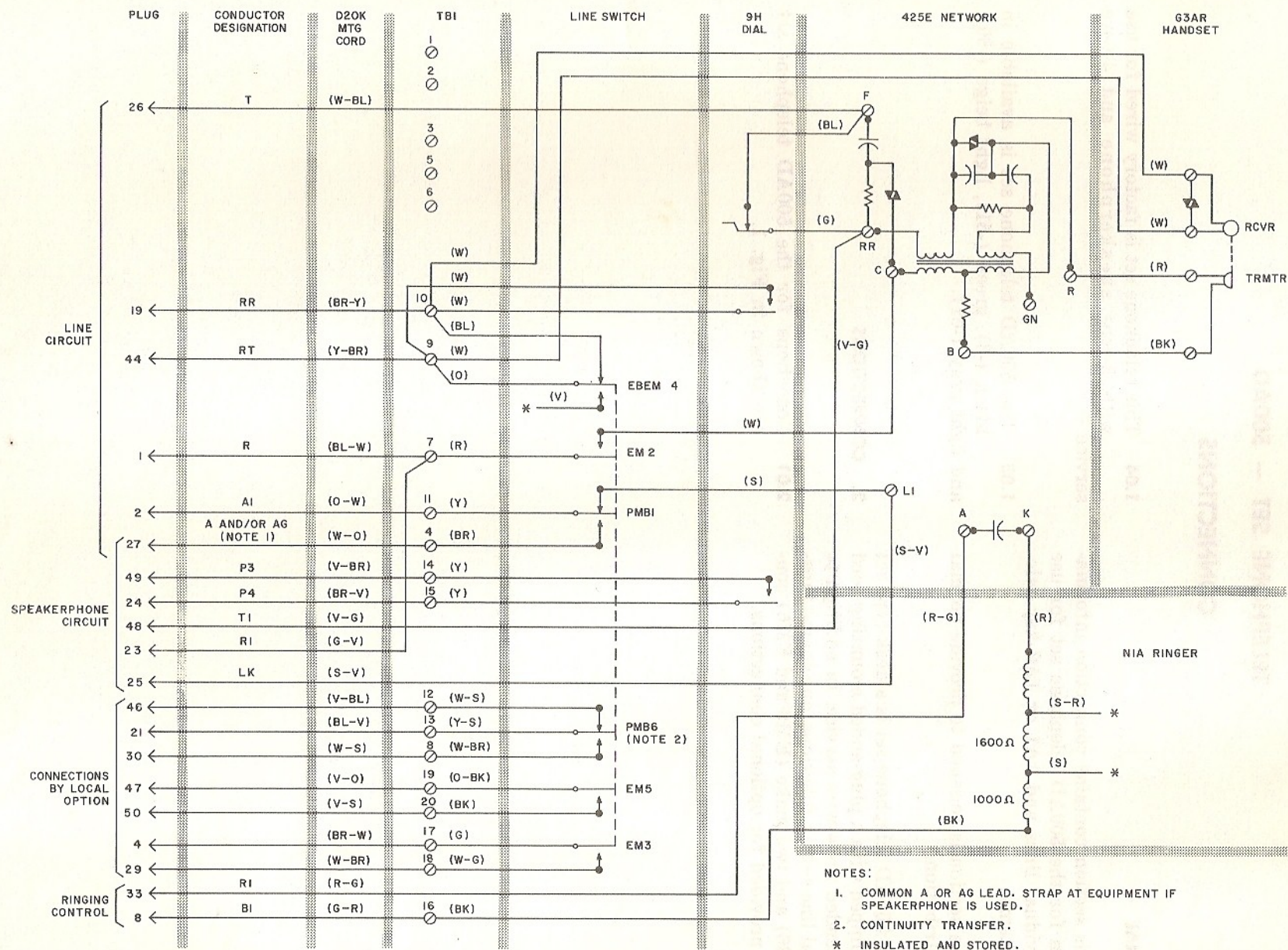
Fig. 1 — 500AD Telephone Set, Connections
