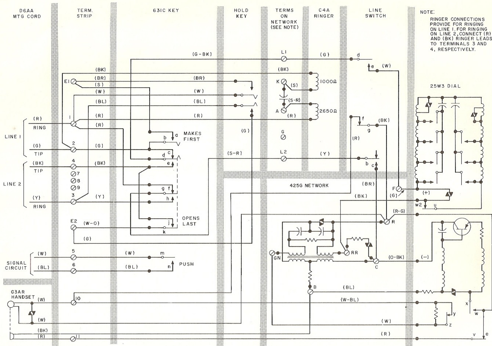
Fig. 2—1515B Telephone Set Connections With 25W3 Dial
