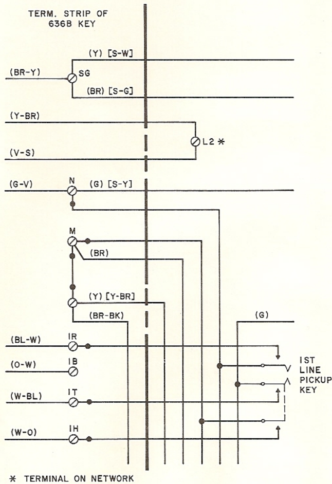
Fig. 2 — Set Wired for 1A Key Telephone System
