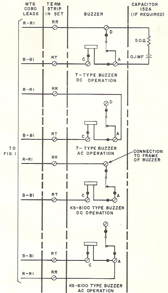
Fig. 3 — Buzzer Connections
