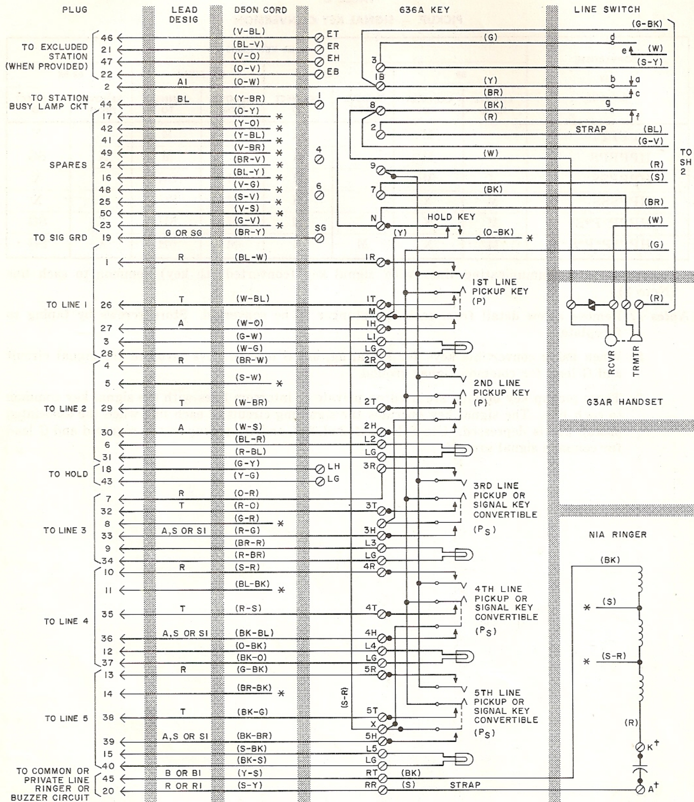
Fig. 1 — 1563HB Telephone Set Using 425G Network and 25W3 Dial, Connections (Sheet 1 of 2)
