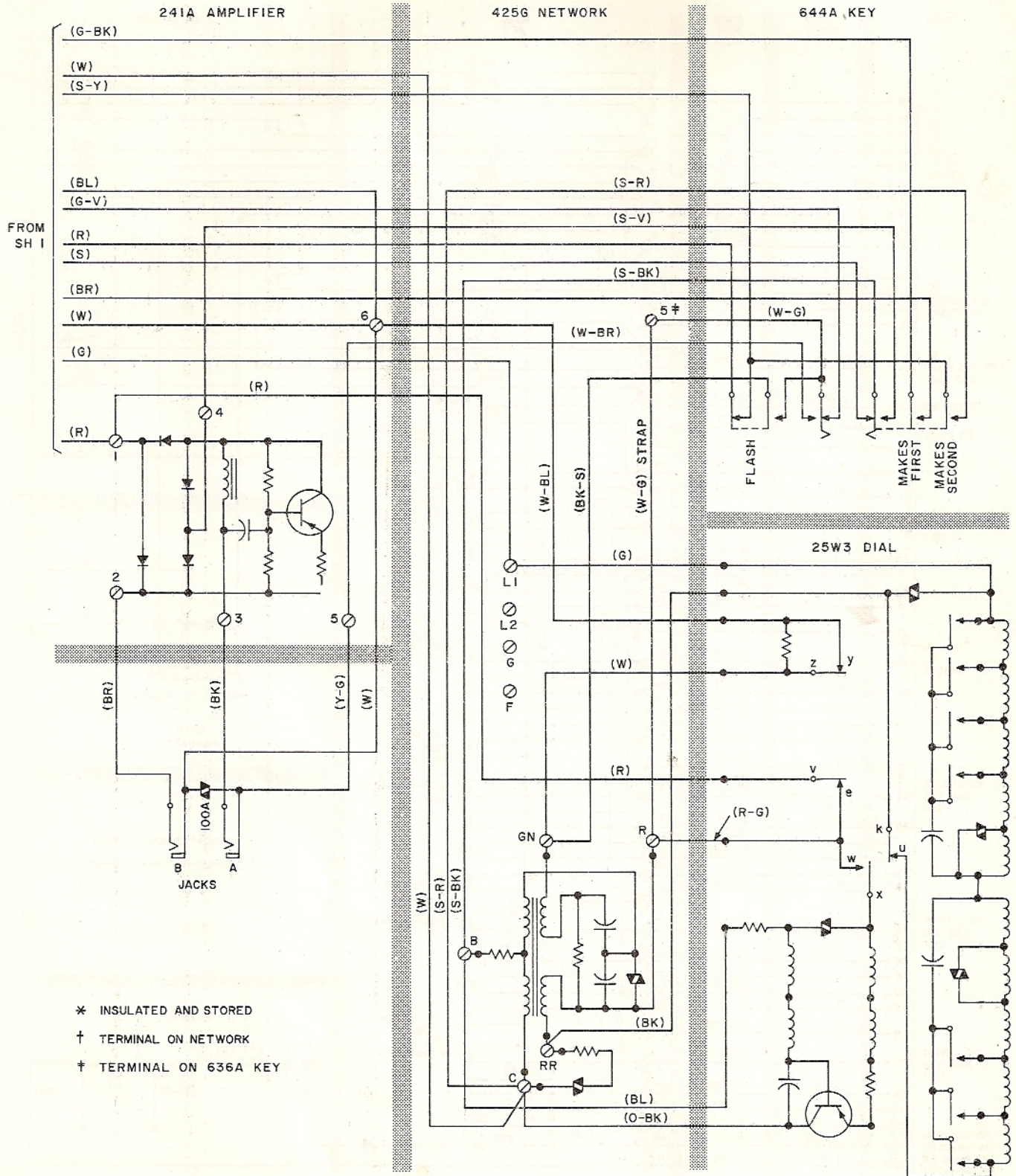
Fig. 1 — 1563HB Telephone Set Using 425G Network and 25W3 Dial, Connections (Sheet 2 of 2)
