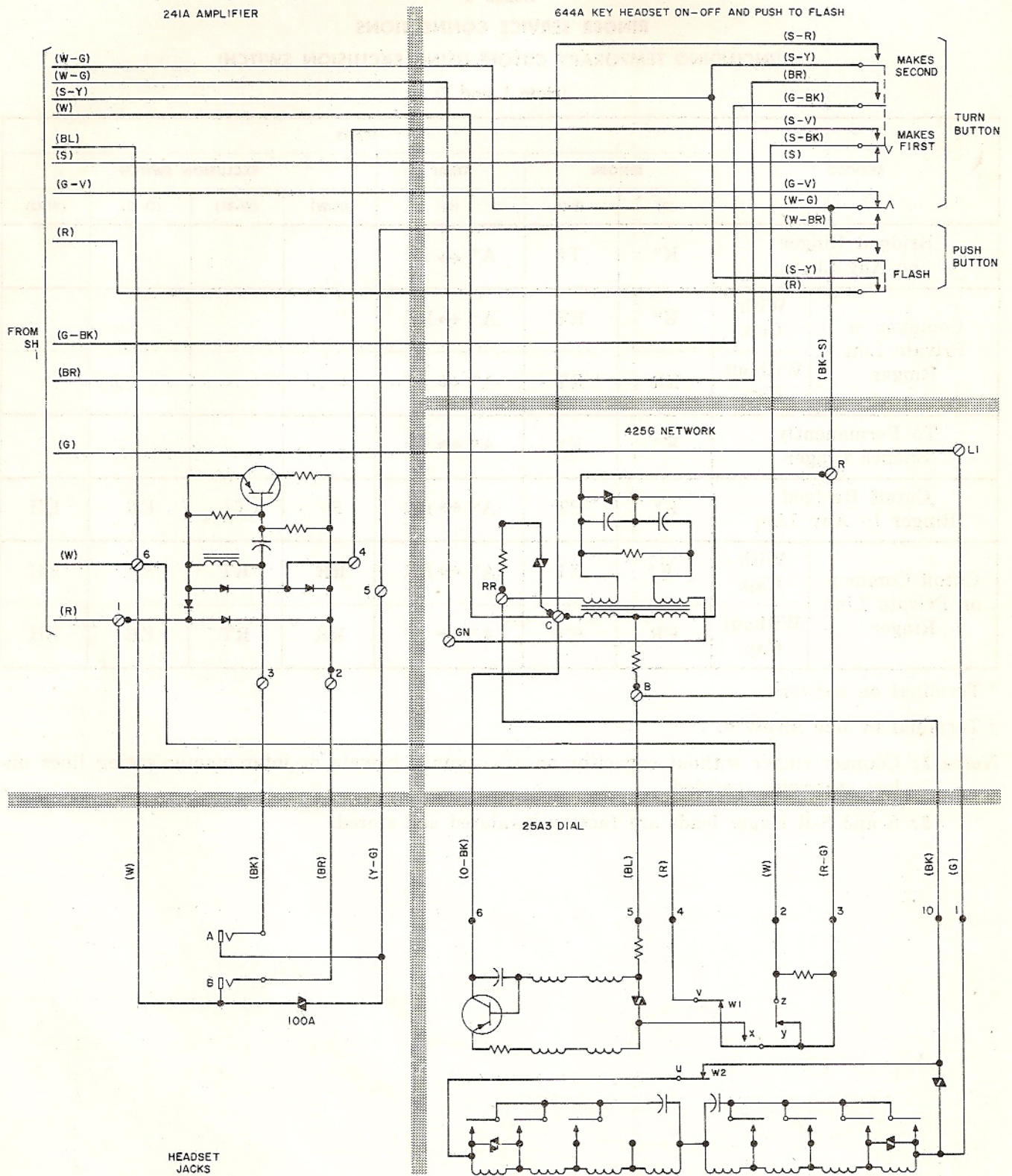
Fig. 2 — 1563HB Telephone Set Using 425G Network and 25A3 Dial, Connections (Sheet 2 of 2)
