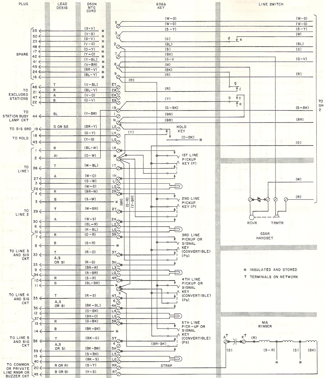
Fig. 2 — 1563HB Telephone Set Using 425G Network and 25A3 Dial, Connections (Sheet 1 of 2)
