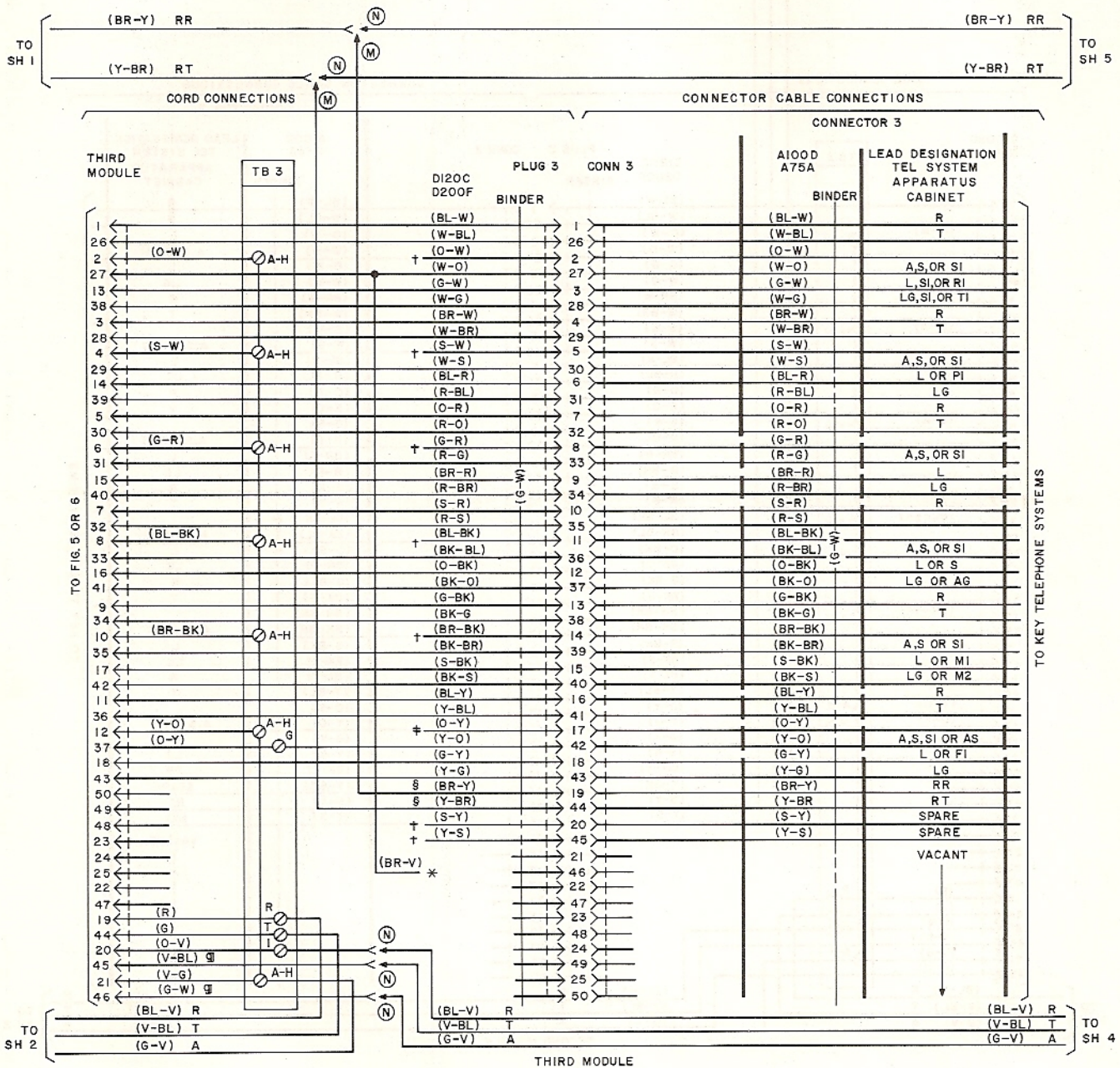
Fig. 8—Cord and Cable Connections (Sheet 3 of 5)
