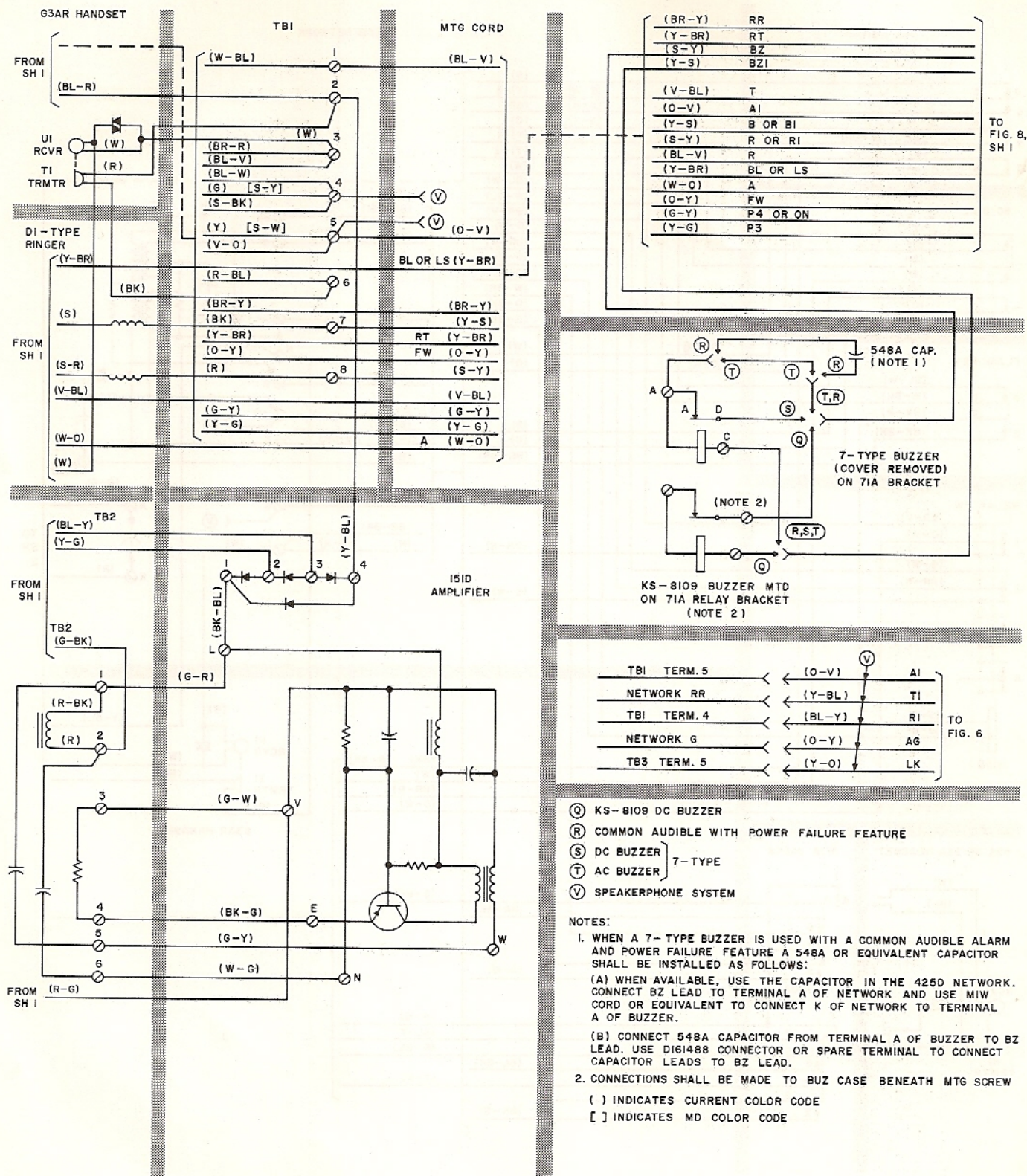
Fig. 1—608B or 618A Telephone Set (Sheet 2 of 2)
