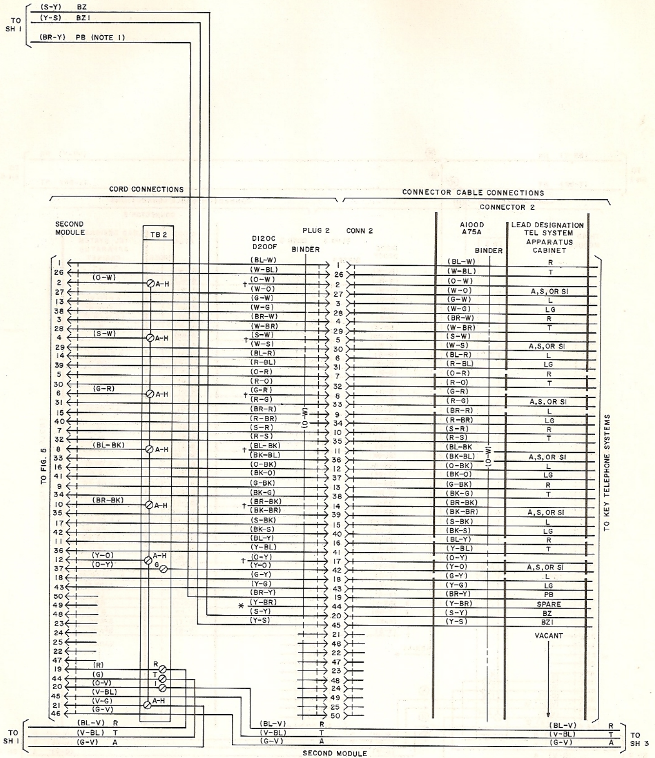
Fig. 8—Cord and Cable Connections (Sheet 2 of 5)
