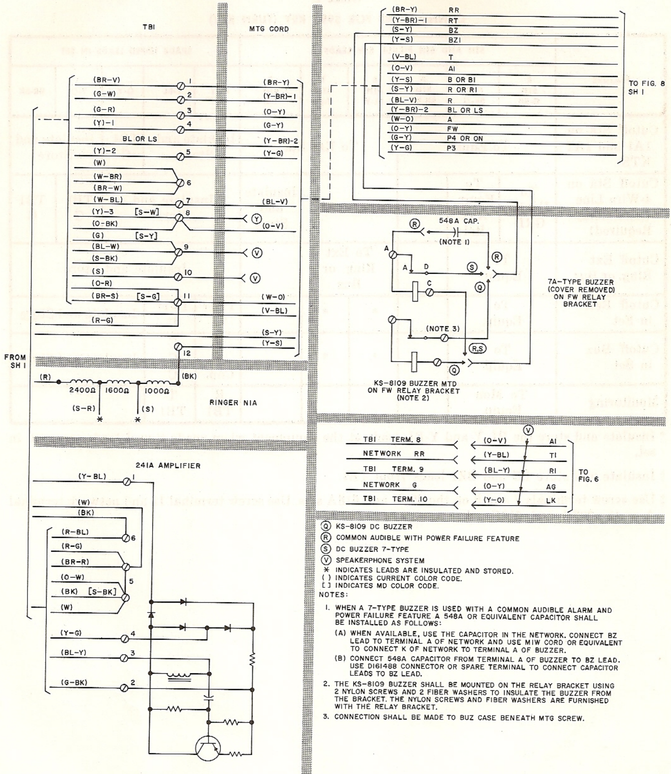
Fig. 2—608C or 618B Telephone Set (Sheet 2 of 2)
