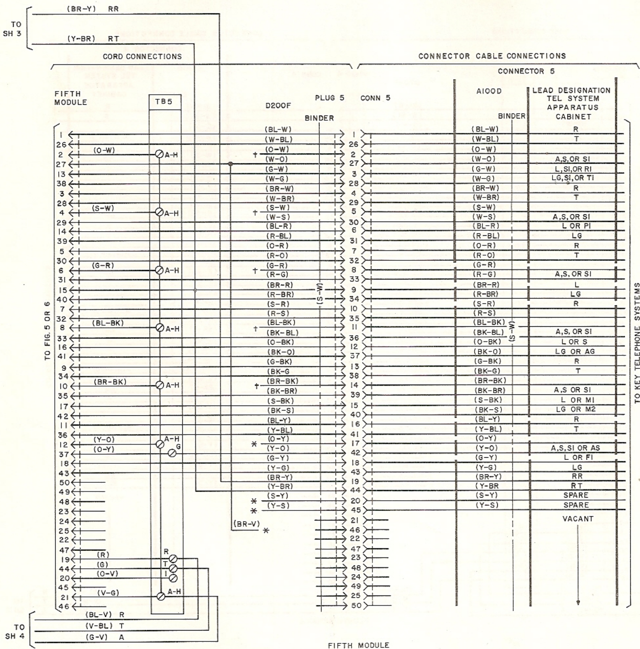
Fig. 8—Cord and Cable Connections (Sheet 5 of 5)
