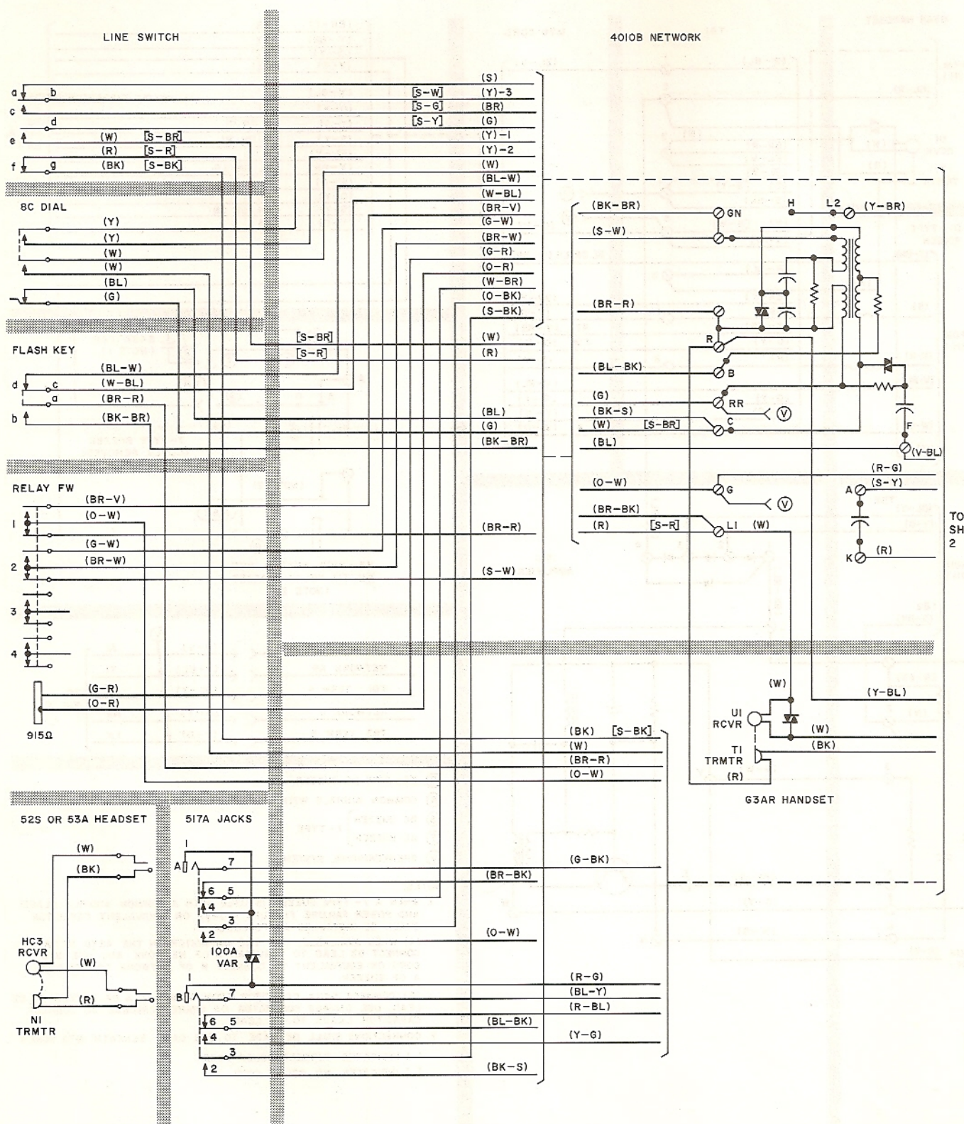
Fig. 2—608C or 618B Telephone Set (Sheet 1 of 2)
