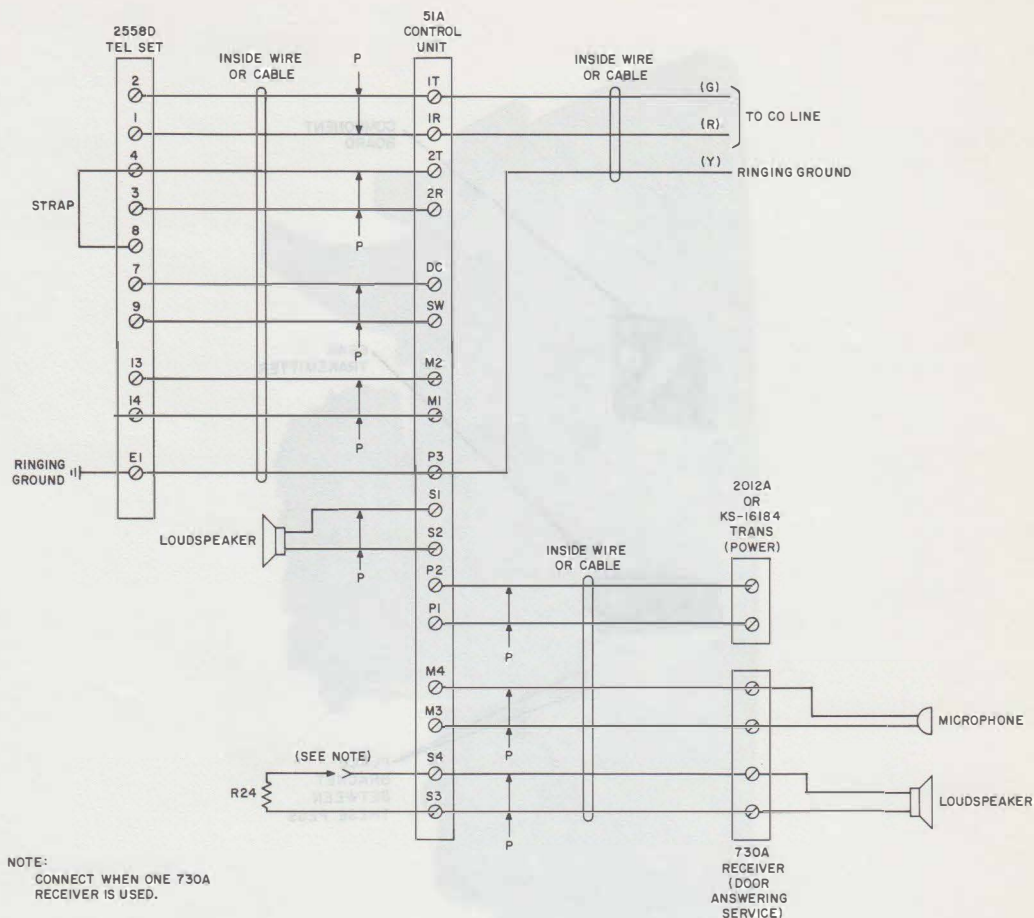
Fig. 2—2558D Telephone Set Connections To 1A Home Interphone
