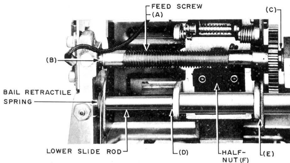
Half-Nut and Feed Screw Details
