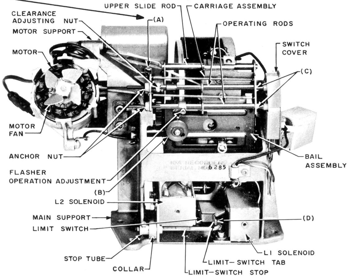
10A Recorder, Front View (Shown at End of Maximum Announcement Interval)
