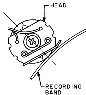
INCORRECT ALIGNMENT
