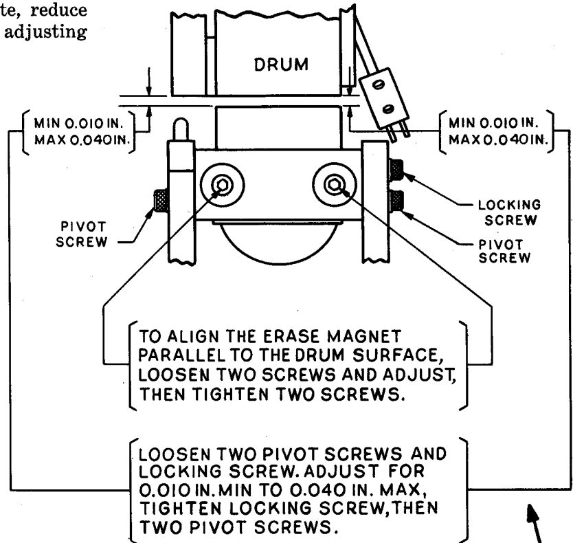
ERASE COIL ASSEMBLY 3.22 (Reqt 2.22)
