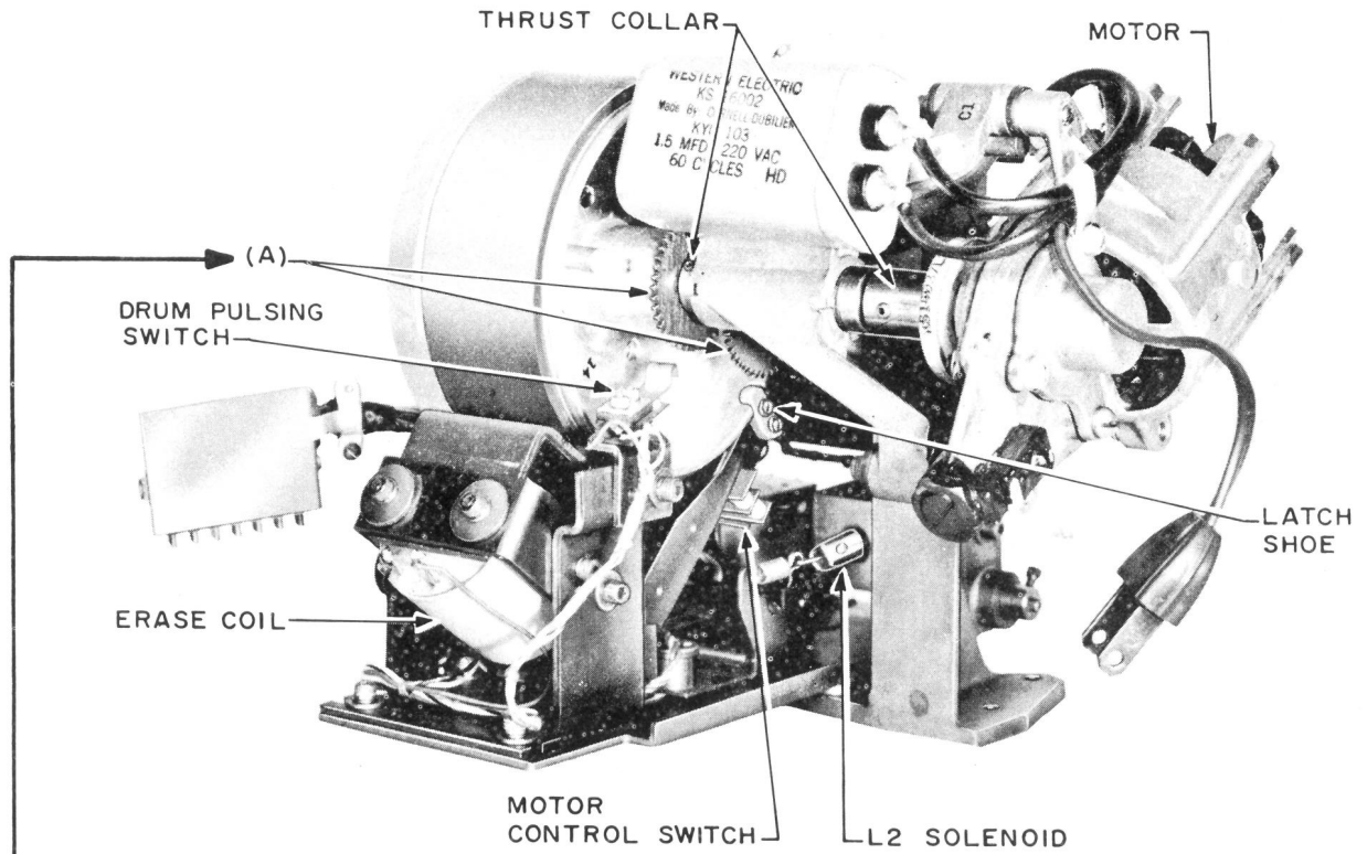
10A Recorder, Rear View
