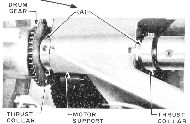
Drum Shaft
