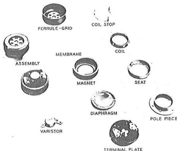
Fig. 8—U1 Receiver Parts
