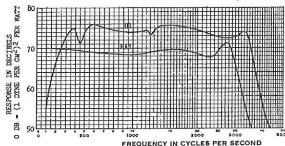
Fig. 9—Available Power Response-Frequency Characteristics of U1 and HA1 Receivers in Standard Handles Measured on a 6-cc Coupler
