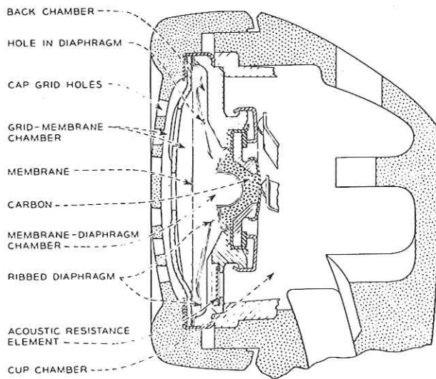
Fig. 5—T1 Transmitter—Sectional View in G1 Handset
