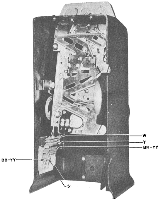
FIG. 3—152C, D—UPPER HOUSING TERMINALS
