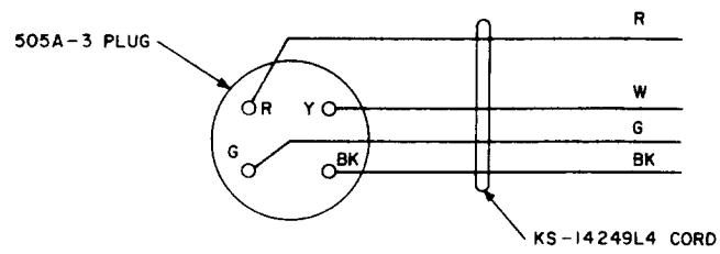
Fig. 10— 505A-3 Plug Connections
