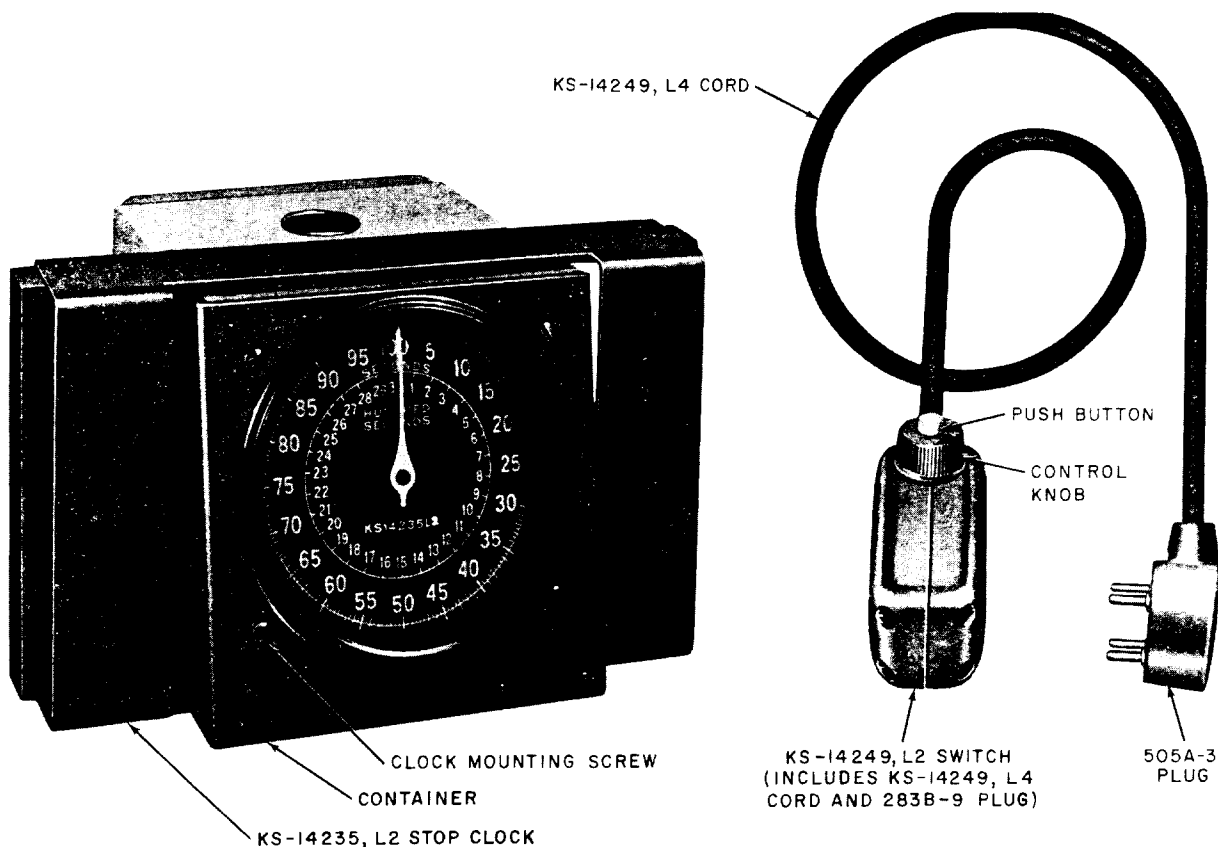
Fig. 9—KS-14235 L2 Stop Clock and KS-14249 L2 Switch
