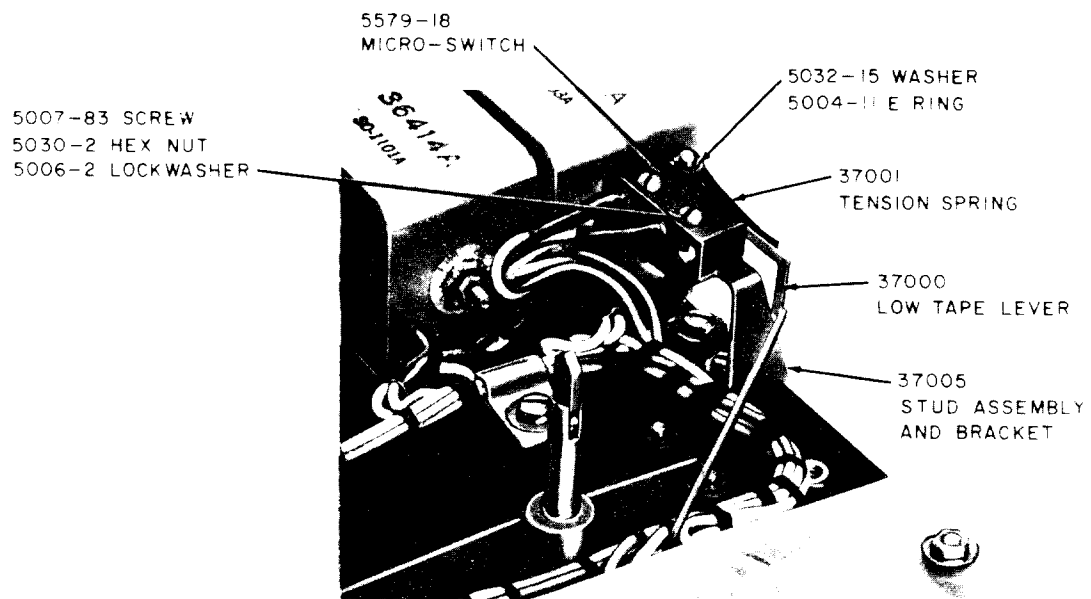
Fig. 4—KS-19717 L10 Low Tape Alarm
