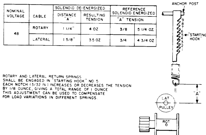
Fig. 8—Rotary and Lateral Return Spring Attachment and Adjustment
