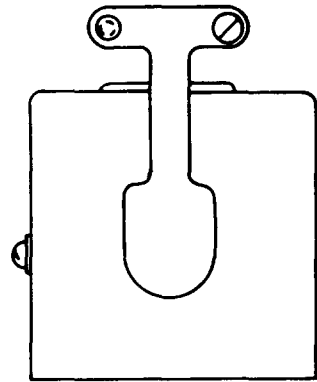
Fig. 14—KS-14525, L4 Connector
