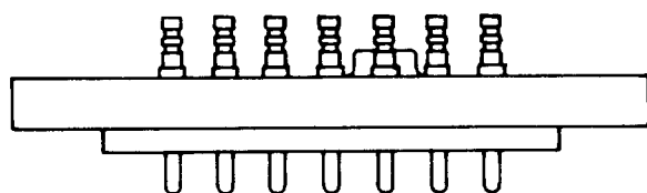
Fig. 8—KS-14380 Connector
