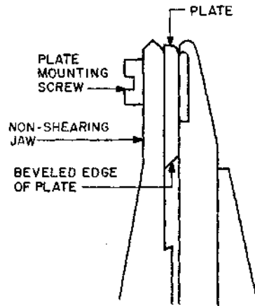
Fig. 2—Plate Mounted on Jaw of 578G Pliers
