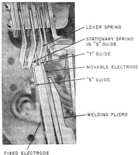
Fig. 11—Welding Contact on Movable (lever) Spring of VON Assembly of 197-Type Switch Using 577A or 577B Welding Pliers
