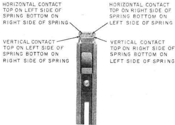
Fig. 8—Fixed Electrode Showing Slot Arrangement
