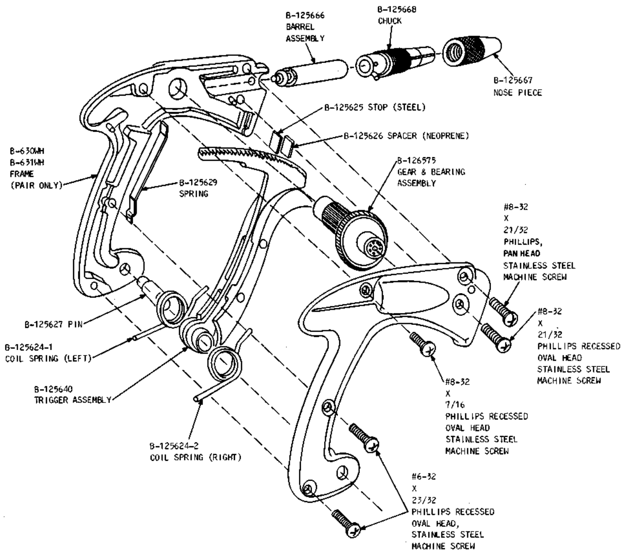
Fig. 2—KS-16363 Wire-Wrapping Tool—Exploded View
