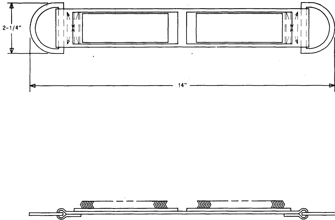
Fig. 1—C Carding Brush
