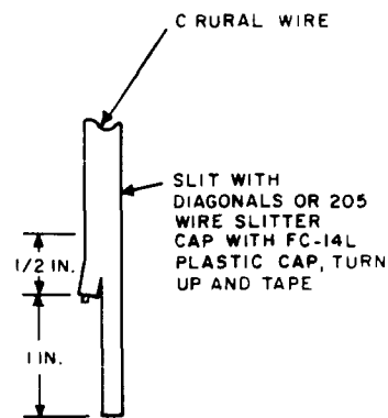
Fig. 2—Preparation of C Rural Wire for FC-14L Plastic Cap
