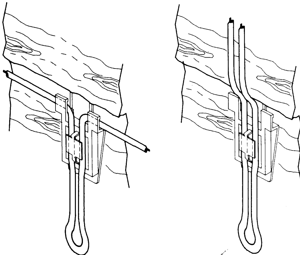
Fig. 6—Double Run of Station Wire Installed Vertically or Horizontally
