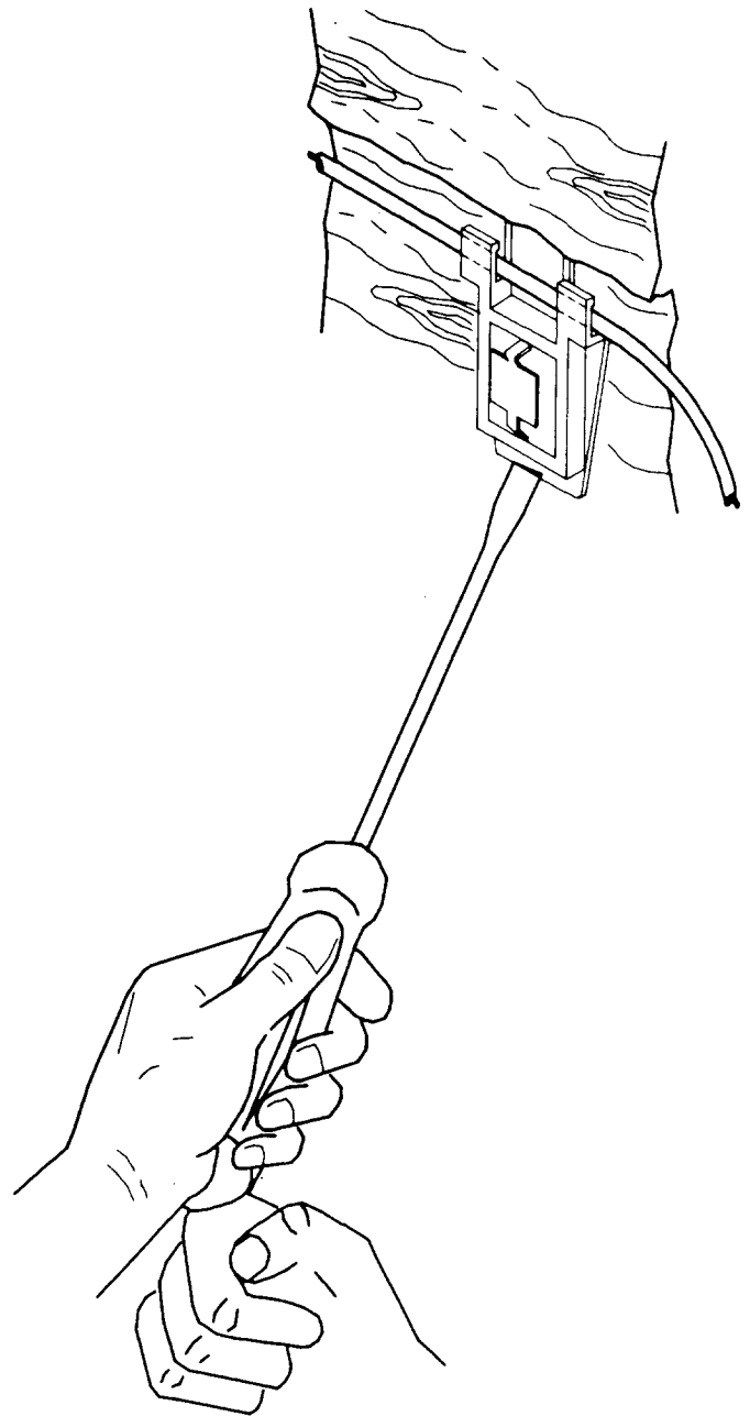
Fig. 4—Installing B Siding Clip
