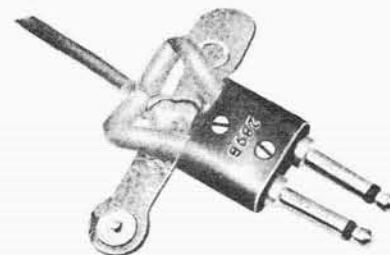
Fig. 9 - 289B Plug - Assembled
