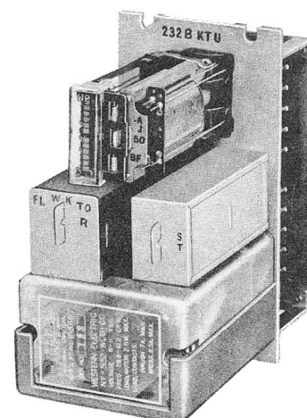
Fig. 17 – 232B KTU, Electro- mechanical Flash, Wink, Ring, and Timeout Circuit
