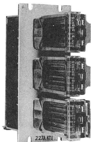
Fig. 15 – 227A KTU Auxiliary Relay Circuit
