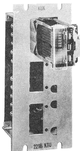
Fig. 16 – 229B KTU, Multiple Line Add-On Transfer Circuit
