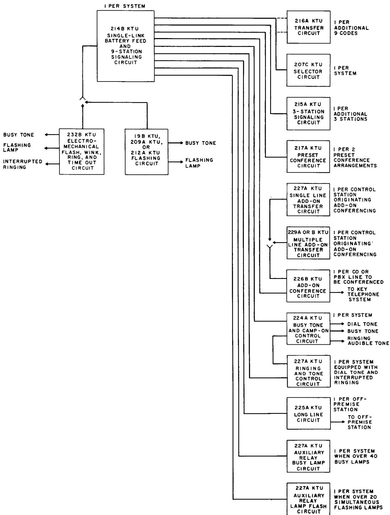
Fig. 2 — Single-Link Arrangement, Using 214B KTU
