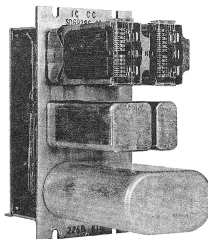
Fig. 14 — 226B KTU, Add-On Conferencing Control Circuit
