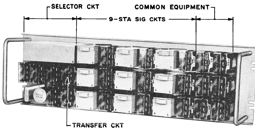
Fig. 18 – 234A KTU, Battery Feed and Signaling (Single-Link) Selector and Transfer Circuit
