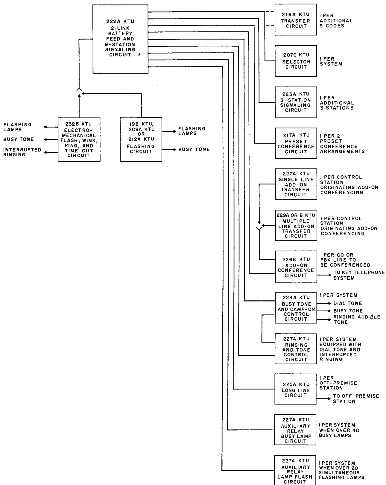
Fig. 4 — Two-Link Arrangement
