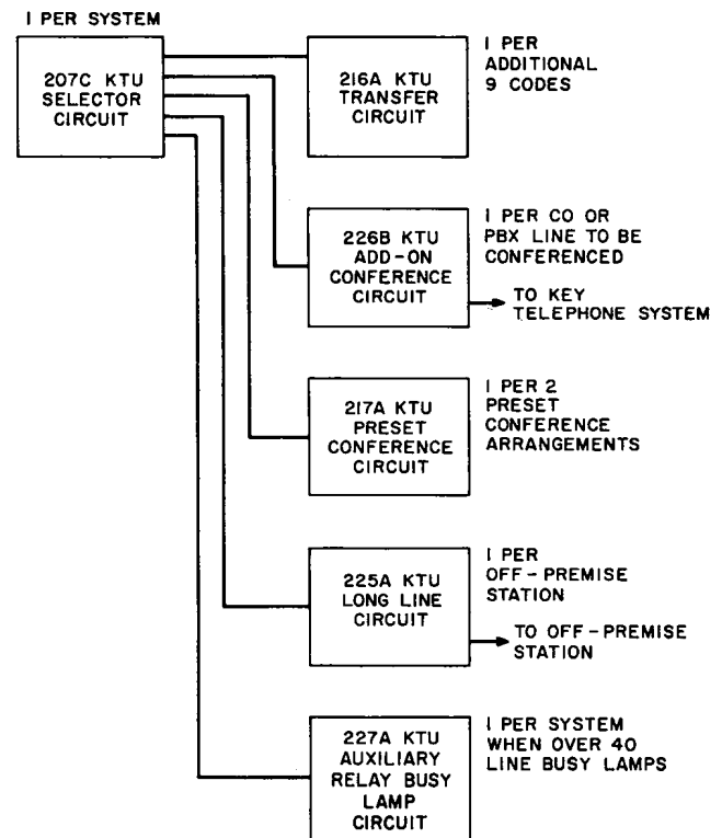
Fig. 1 — Selector-Only Arrangement
