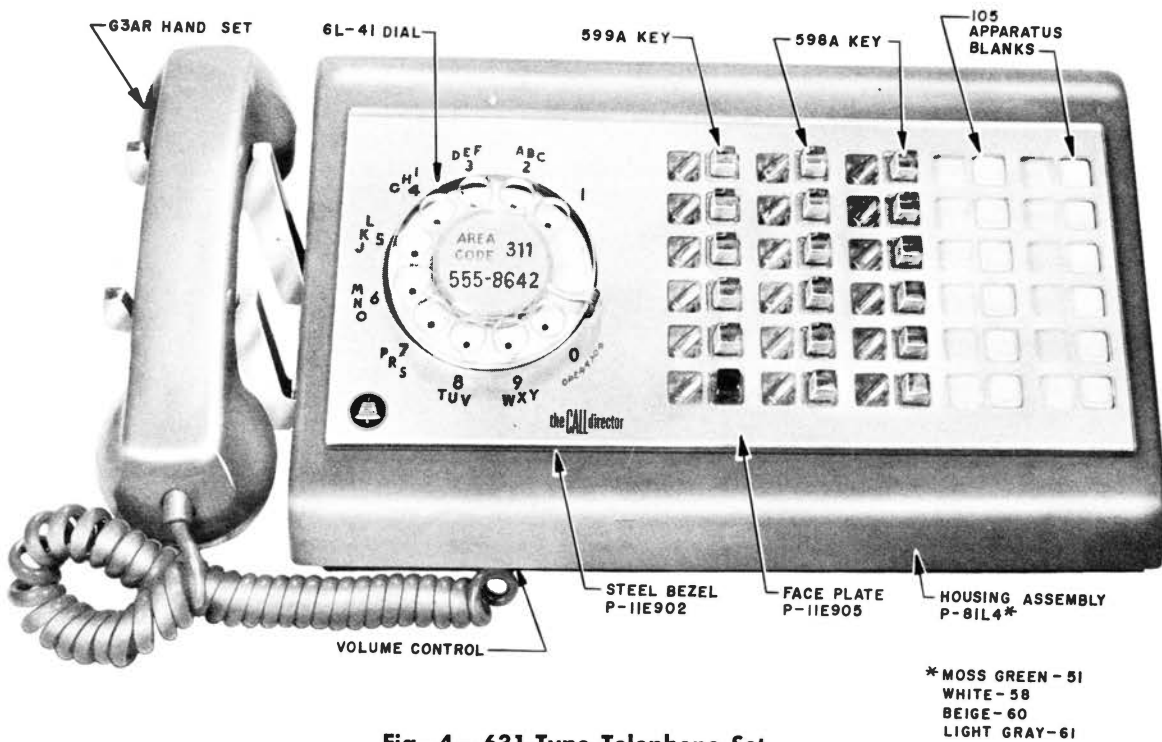
Fig. 4 — 631-Type Telephone Set
