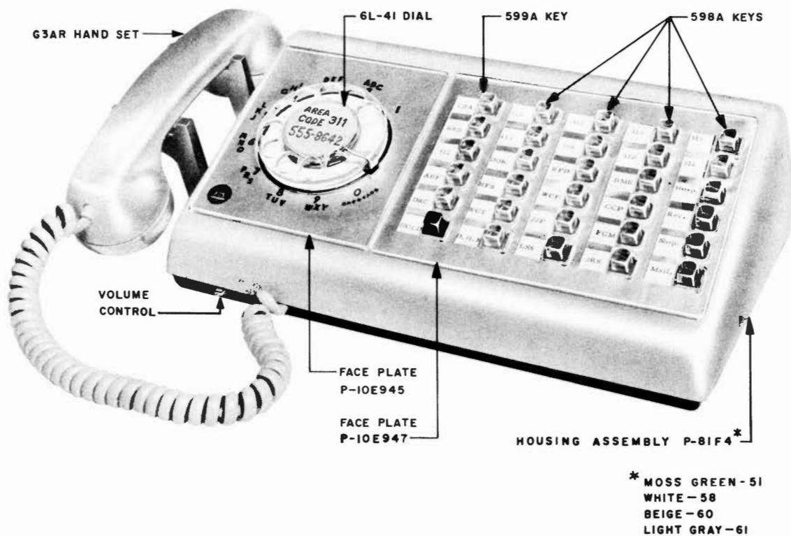
Fig. 2 — 601-Type Telephone Set
