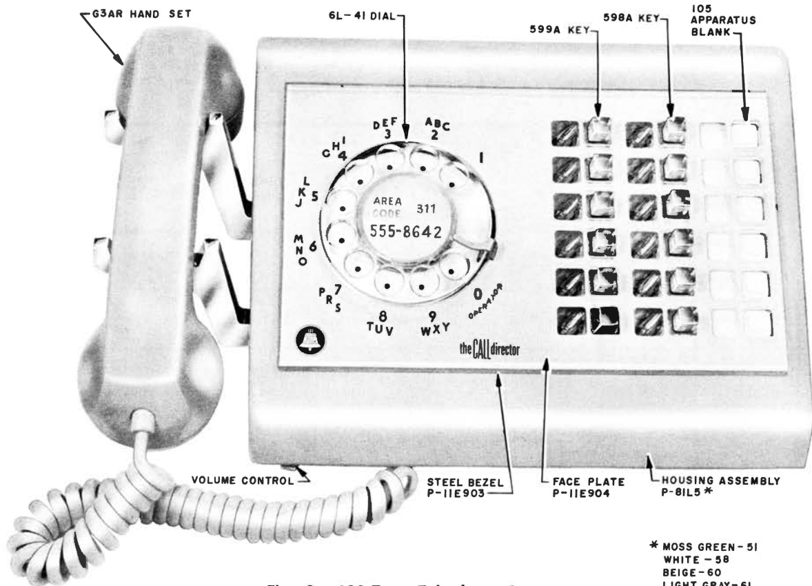
Fig. 3 — 630-Type Telephone Set
