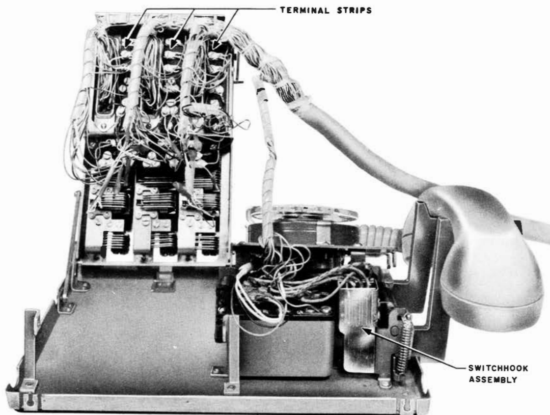
Fig. 15 — 600-Type Telephone Set, Key Frame Lifted, Rear View
