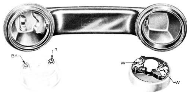
FIG. 3—G1-TYPE HANDSET
