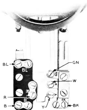
FIG. 5—G6-TYPE HANDSET MOUNTING
