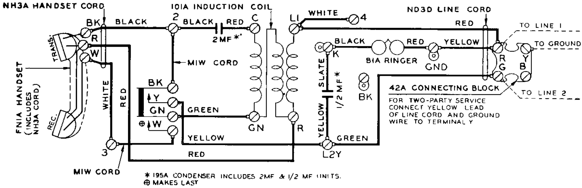
Wiring Diagram for No. 1 Type Uniphone for Manual Service
